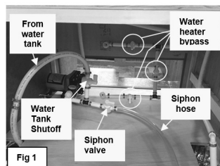
Water valves and water heater bypass
