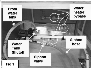
Water valves and water heater bypass
